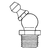
65° 1/8 Pipe Thread
